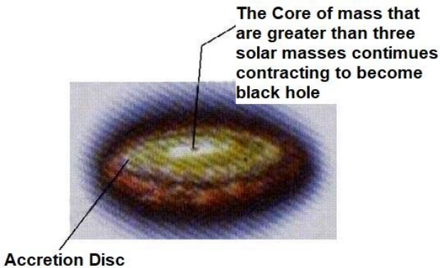
FIGURE 6.5: Formation of Black Hole
