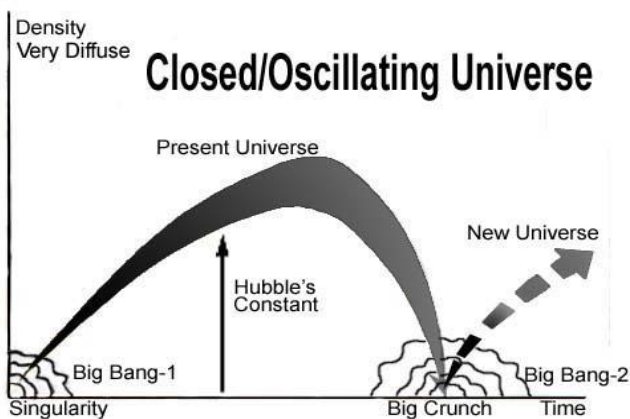
FIGURE 9.1: Cyclic Universe
