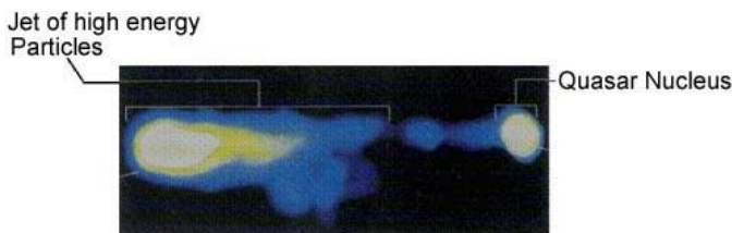
FIGURE 6.12: Quasar (3C273)
