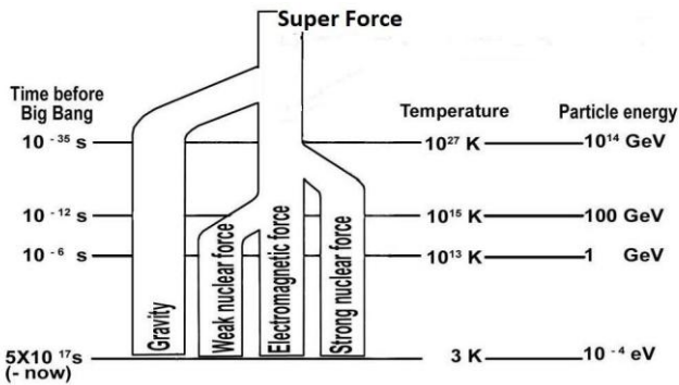
FIGURE 3.2: GUT Forces
