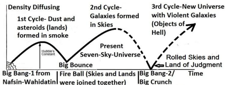
FIGURE 8.1: Cyclic Universe
