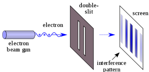
FIGURE 3.3: Double-slit Experiment
