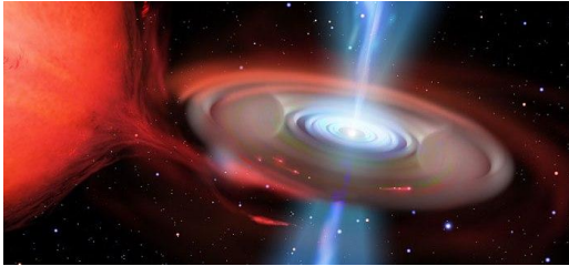
FIGURE 6.6: Black Hole
