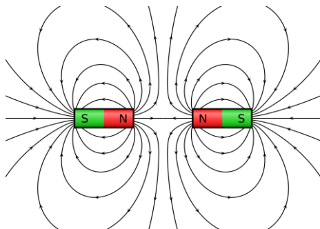
FIGURE 2.8: Magnetic Field
