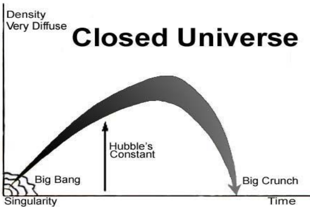
FIGURE 4.2: Closed Universe
