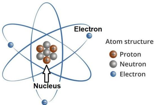
FIGURE 2.11: Atom
