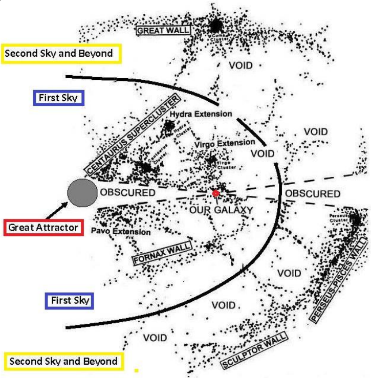
FIGURE 2.20: Likely First and Second Sky
