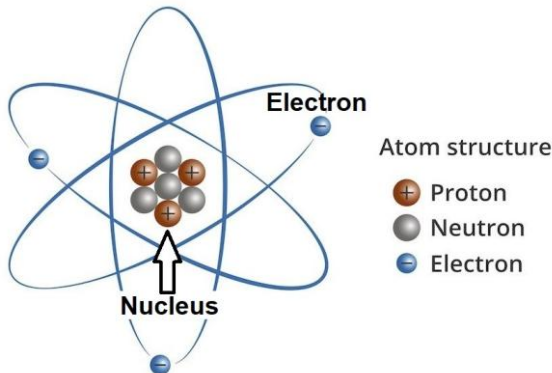
FIGURE 1.8: Atom
