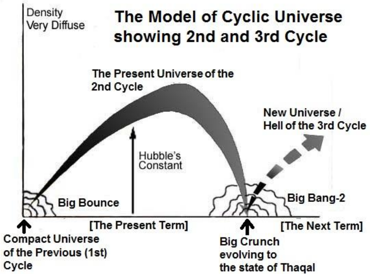
Figure 6.1: Evolution of Universe
