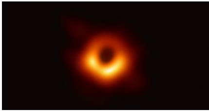
FIGURE 3.11: A Black Hole
