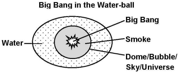
FIGURE 3.1: Water and Big Bang
