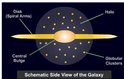
FIGURE 3.23: Three Basic Components of a Spiral Galaxy
