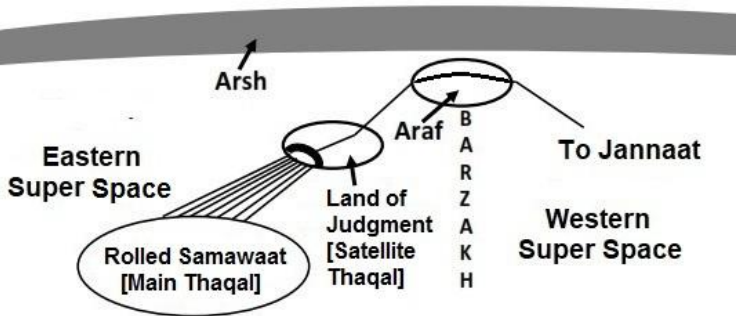
FIGURE 1.16: Super Space
