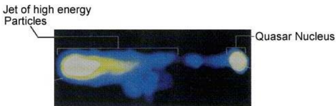
FIGURE 3.15: Quasar (3C273)
