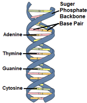
FIGURE 6.5: The Noble Pair (Double Helix DNA Molecule)
