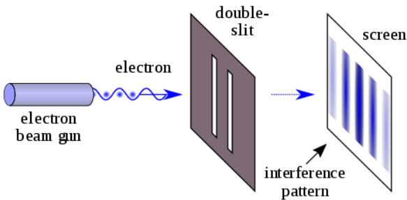
FIGURE 1.9: Double-slit Experiment
