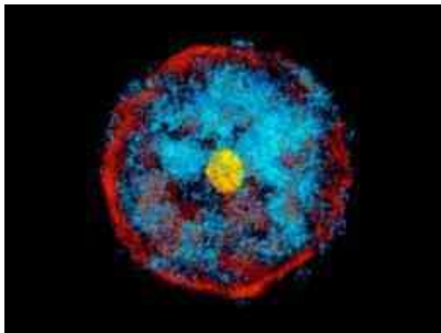
FIGURE 3.3: The Red Giant
