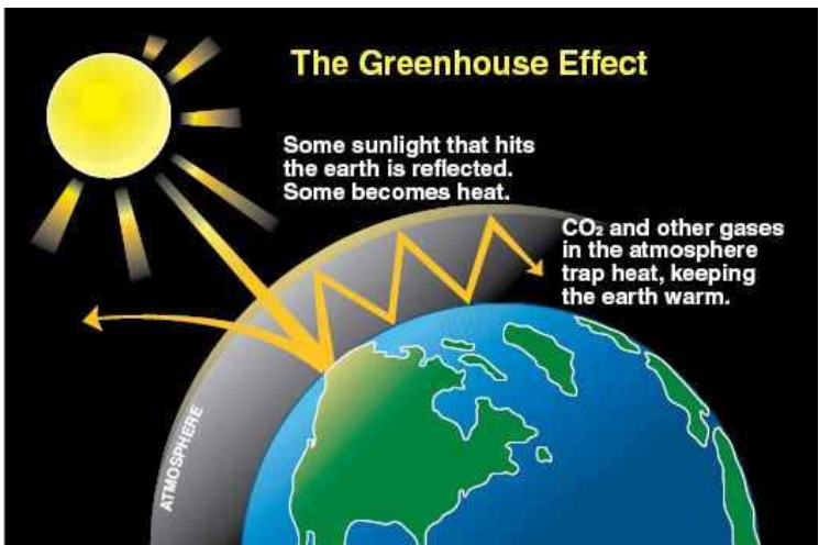
FIGURE 2.3: Greenhouse Effect
