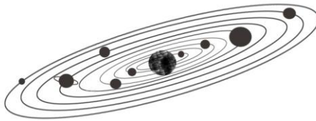
FIGURE 2.7: The Solar System
