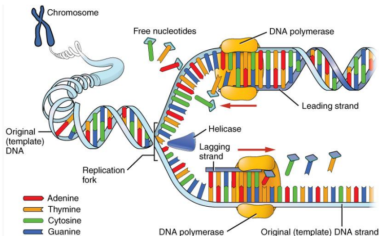
FIGURE 6.8: DNA Replication
