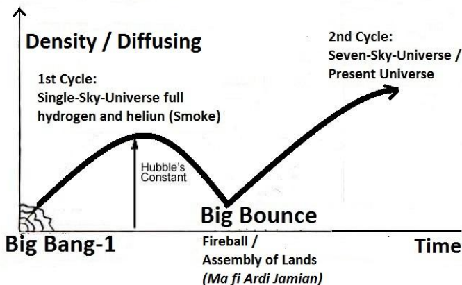
FIGURE 2.6: Big Bounce
