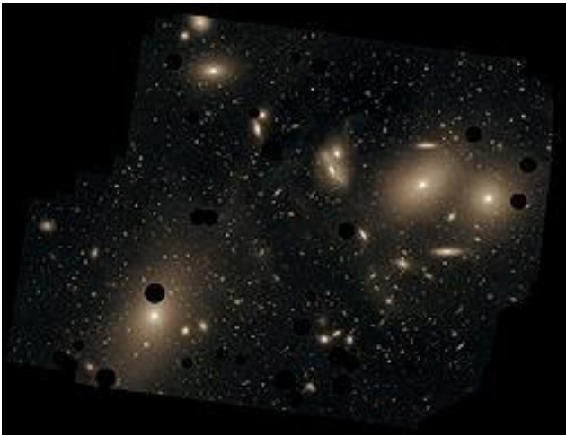
FIGURE 2.16: Cluster Virgo
