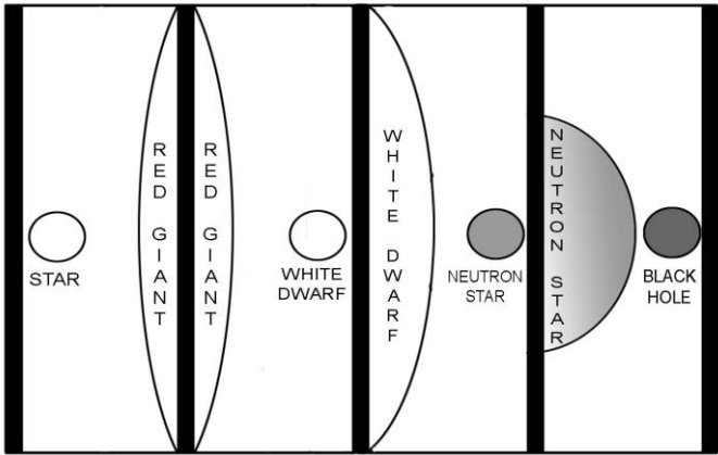
FIGURE 3.12: Stages of Collapsing Star
