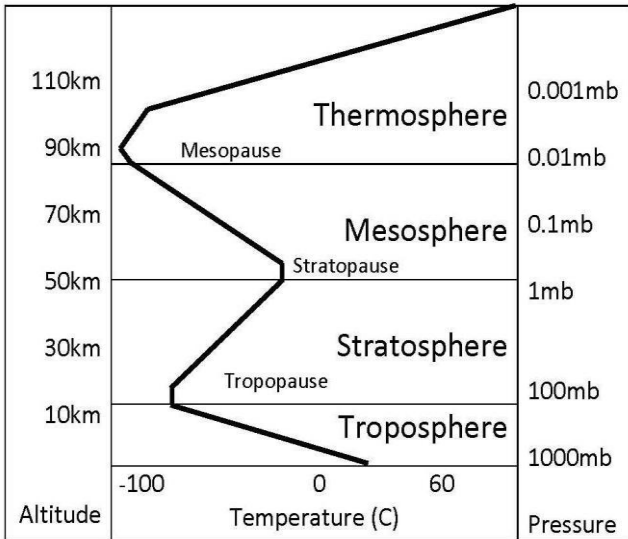
FIGURE 2.5: Temperature Curve
