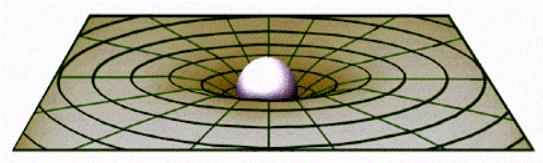
FIGURE 2.17: Curvature of space in two dimensional view
