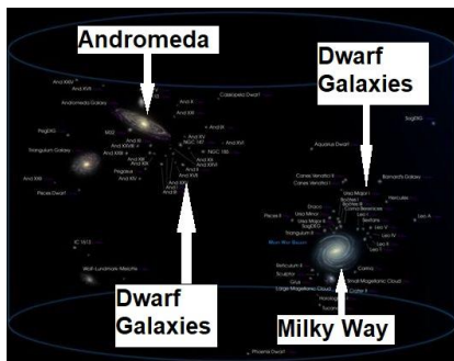
FIGURE 2.15: Local Group
