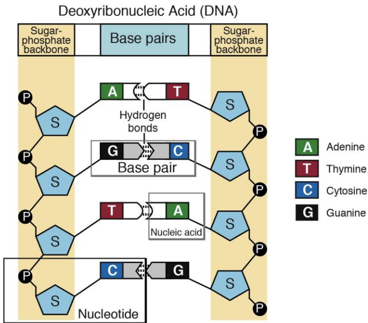
FIGURE 6.7: Double Helix Bondage
