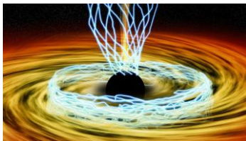
FIGURE 3.18: Accretion Disc / a Crucible
