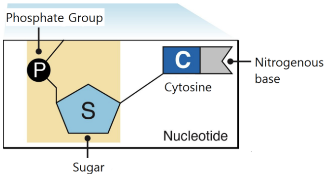
FIGURE 6.6: Nucleotide
