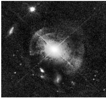
FIGURE 3.14: Quasar MC2 1635+119
